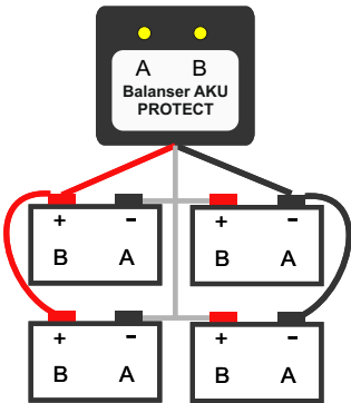
Installation: Battery 24V, 4 batteries
