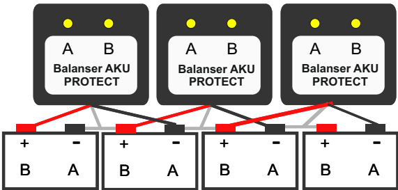
Installation: Battery 48V
