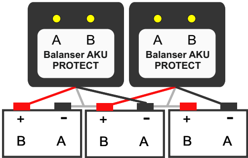
Installation: Battery 36V
