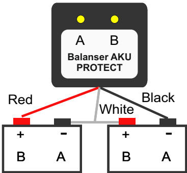
Installation: Battery 24V, 2 batteries
